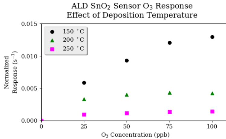
Figure 2. Normalized response to ozone concentration as a function of ALD deposition temperature.
