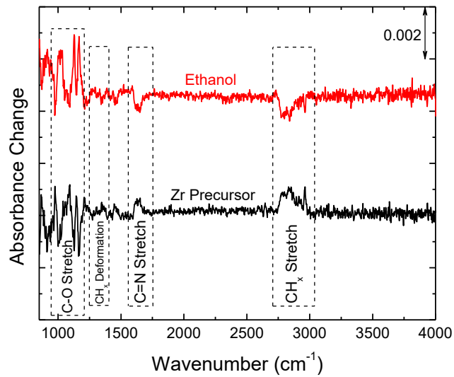
Figure 2. Infrared absorbance change during the TEMAZ and ethanol half-cycle at a substrate temperature of 200 °C.
