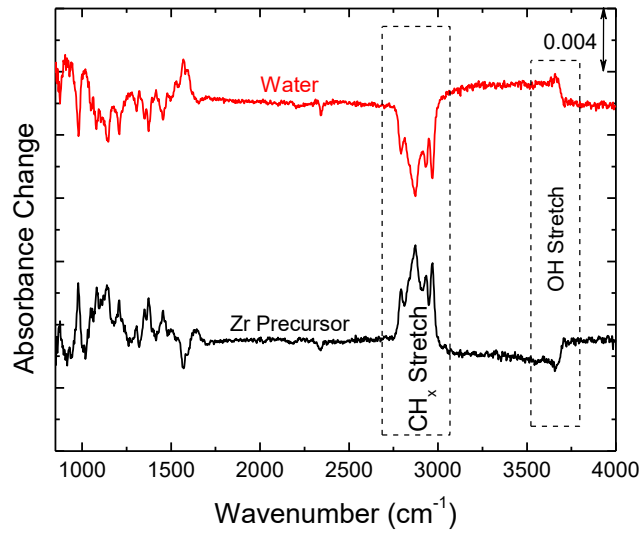
Figure 1. Infrared absorbance change during the TEMAZ and water half-cycle at a substrate temperature of 200 °C.
