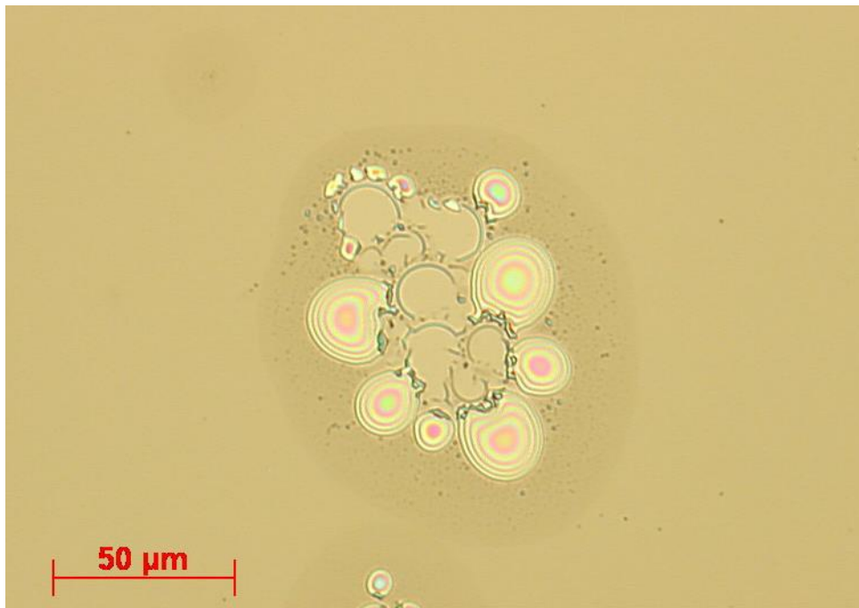
Fig. 1: Microscope image of a boron oxide film capped with antimony oxide after contact to air.
