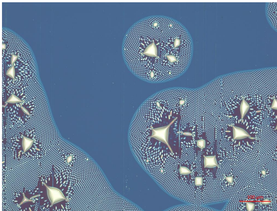
Fig. 2: Microscope image of a phosphorus oxide film capped with antimony oxide after contact to air.
