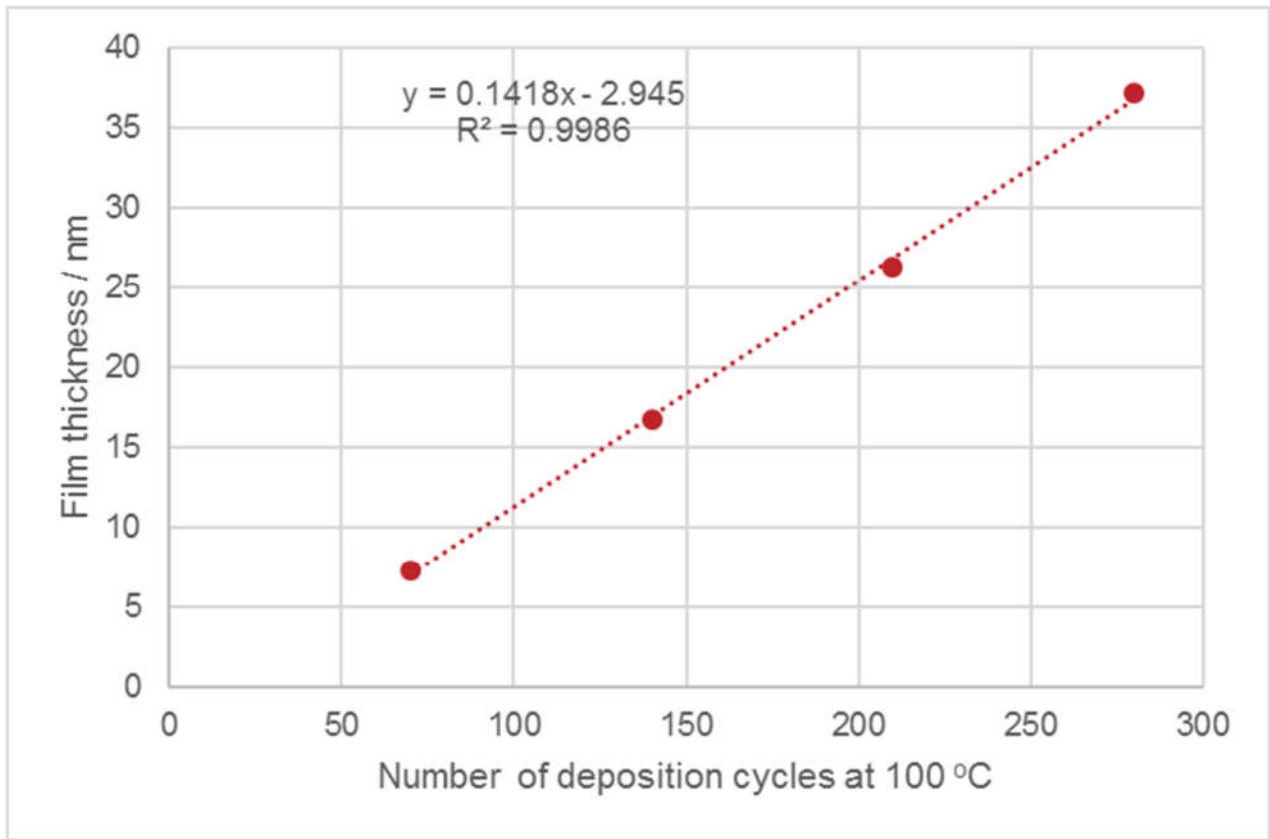
Figure 1: SiO 2 thickness series at 100 °C. Nucleation delay of 21 cycles. Refractive index fixed at 1.457.
