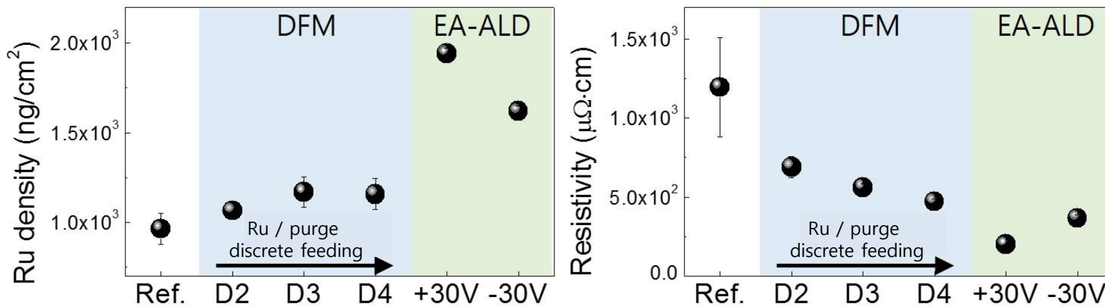
Fig.2 Film layer density and resistivity of Ru film with DFM and EA-ALD.
