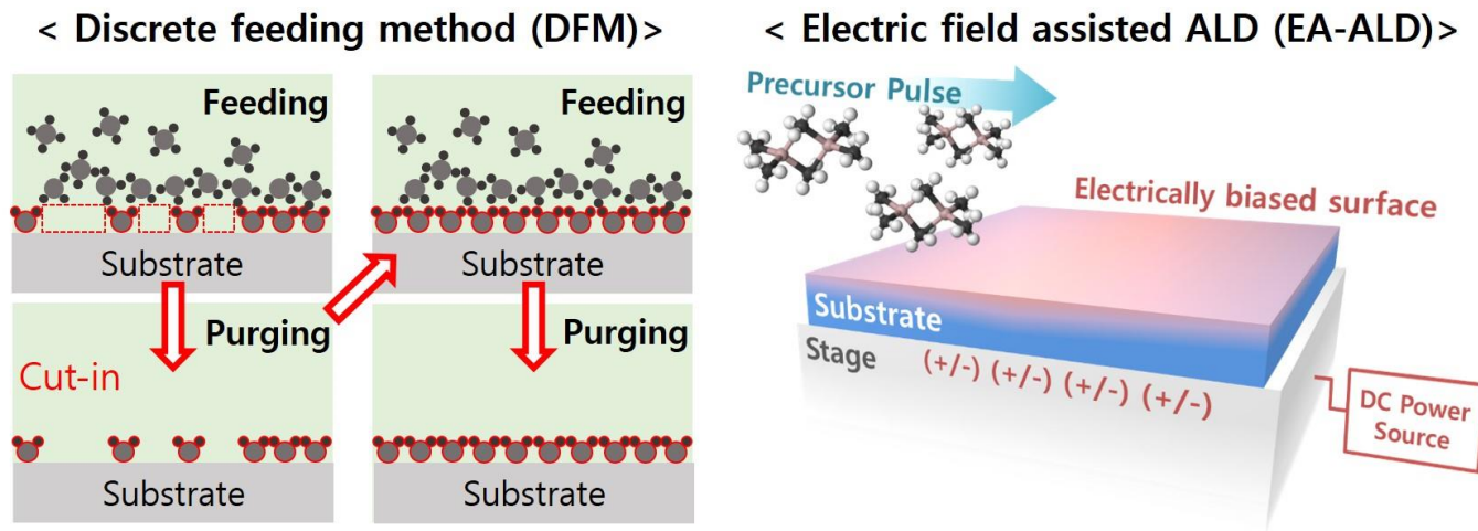
Fig.1 Schematic of DFM and EA-ALD
