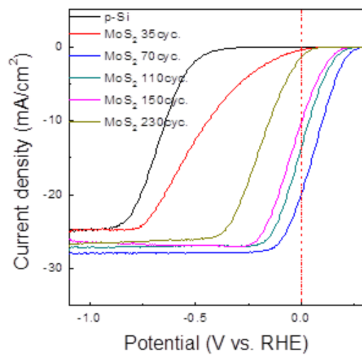
Figure 1. PEC performance of MoS 2 /p-Si photocathodes.
