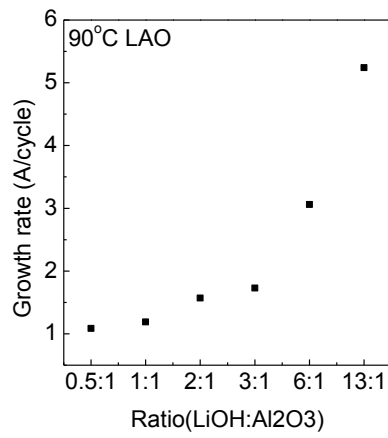
Figure 1 Growth rate of LiAlO films with various compositions.
