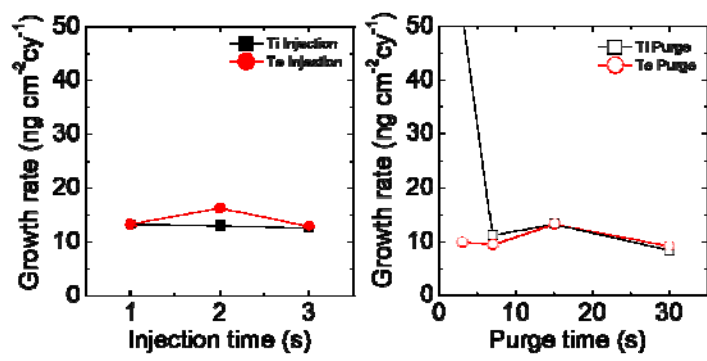
Figure 1. ALD saturation curve of TiTe 2
