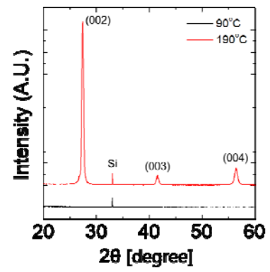
Figure 2. Theta-two theta XRD of ALD TiTe 2
