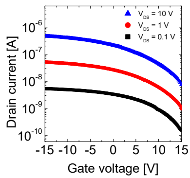
Figure 3. Transfer curves of the TFT
