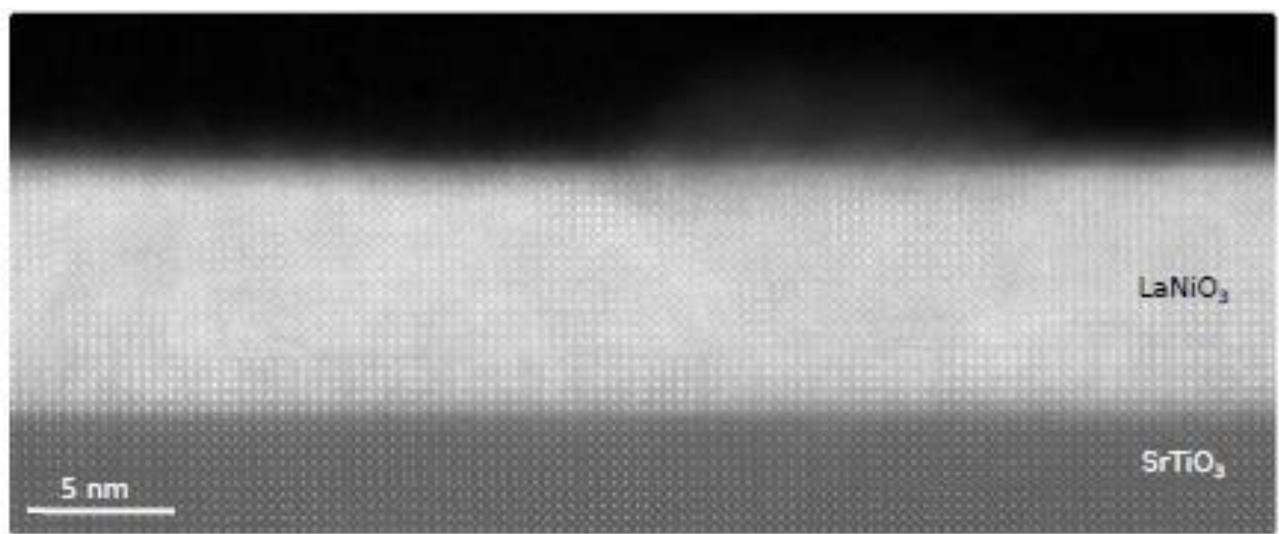
Figure 1: 8.5 nm LaNiO 3 layer deposited on SrTiO 3 by atomic layer deposition.
