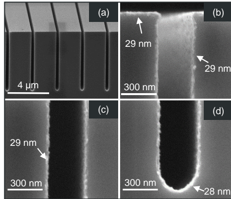
Supplemental Figure 1) SEM images of conformal Te ALD coated trenches using a TeO 2 nucleation seed layer: (a) shows the full 250 nm wide, 24:1 aspect ratio trenches, (b) shows a magnified image of the top of the trench, (c) shows the middle of the trench ~3μm from top, and (d) shows the bottom of the trench.
