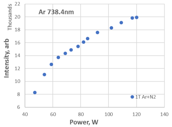
Fig. 4. Argon emission increases with power
