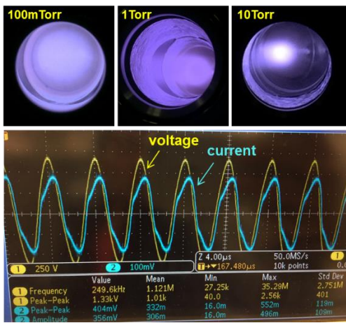
Fig. 3. Plasma generation with various pressures
