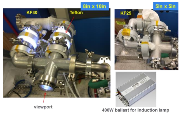
Fig. 2. Prototype chambers and electronic ballast
