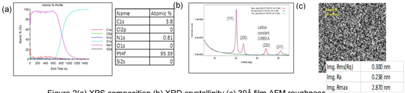
Figure 2(a) XPS composition (b) XRD crystallinity (c) 30Å film AFM roughness
