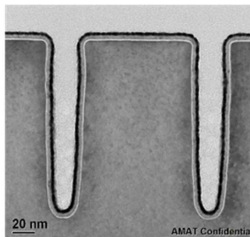
Figure 3: >95 % step coverage for 30Å Pt on TiN films at 130 °C
