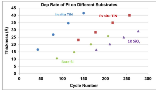
Figure 1: Film thickness of Pt on different substrates showing preference for
