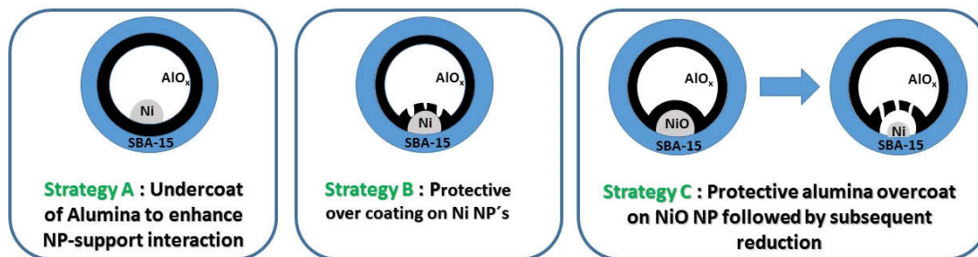
Figure 1. Strategies to modify the supported nickel nanoparticles in mesoporous of SBA 15 using atomic layer deposition
