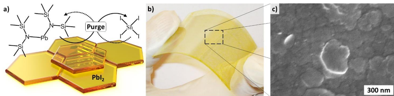
Figure 1. a) Structures of the precursors, b) Pbl 2 film deposited on ITO:PET substrate, c) FESEM image of the same film.
