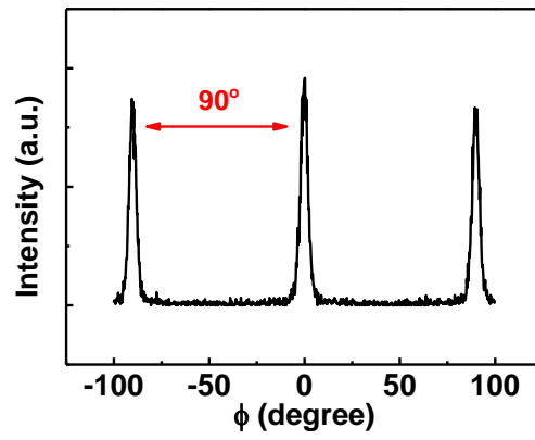
Figure.2 Off-normal \phi -cone scan across YDH{111}
