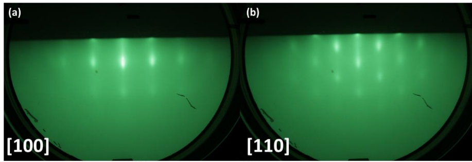
Figure.1 RHEED patterns of ALD-YDH along (a) [100] and (b) [110] direction
