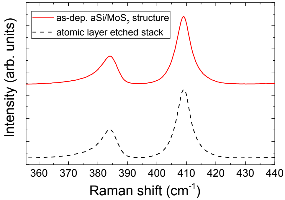
Figure 1: Raman spectra of the MoS 2 related E 2g 1 and A 1g peaks showing the preservation of the MoS 2 after ALE with long overetching
