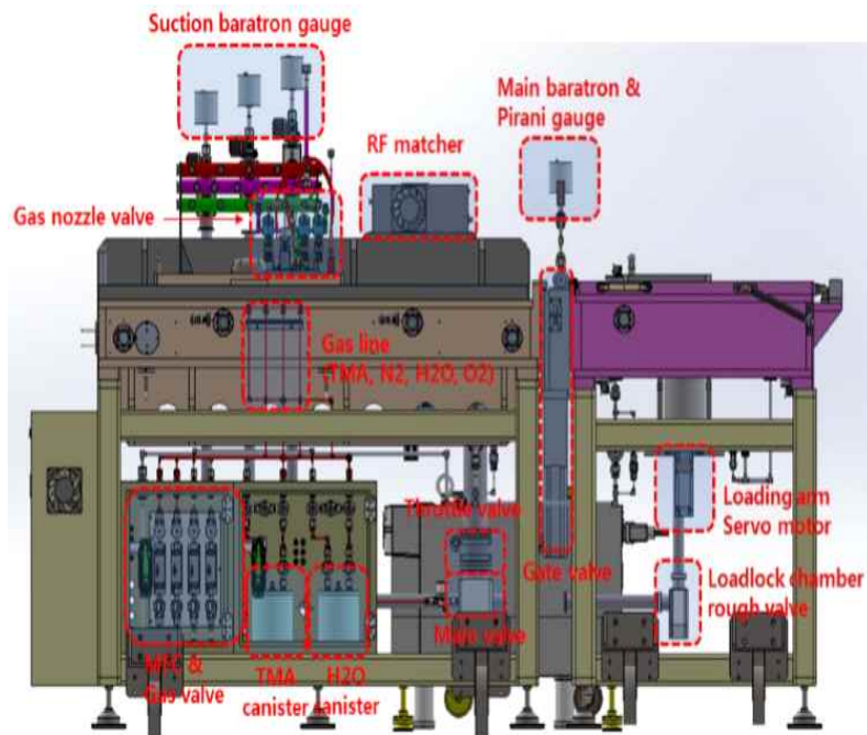
STD-PEALD equipment developed in this study
