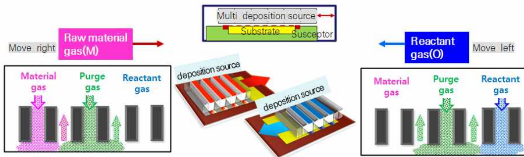
Schematic of the Spatial ALD and STD ALD
