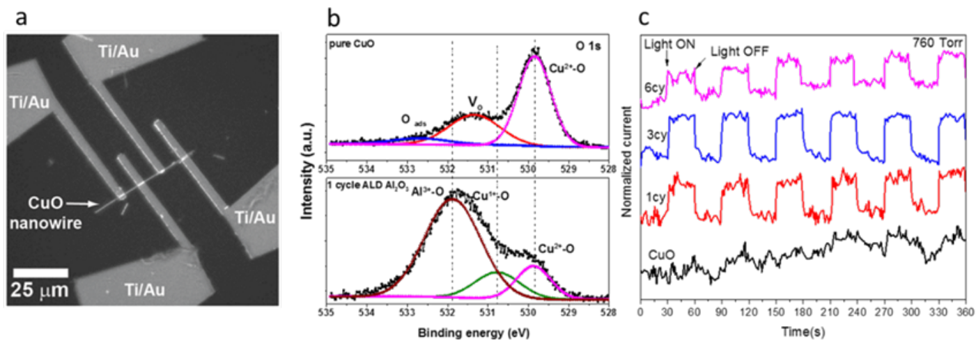
Figure 1 a) CuO nanowire contacted by Ti/Au contacts, b) Oxygen 1s XPS spectra showing the reduction of CuO to Cu 2 O after 1 cycle of ALD c) Chopped current-time characteristic shows a photoresponse on CuO nanowire after 1 ALD cycle compared to negligible photoresponse on pristine CuO.
