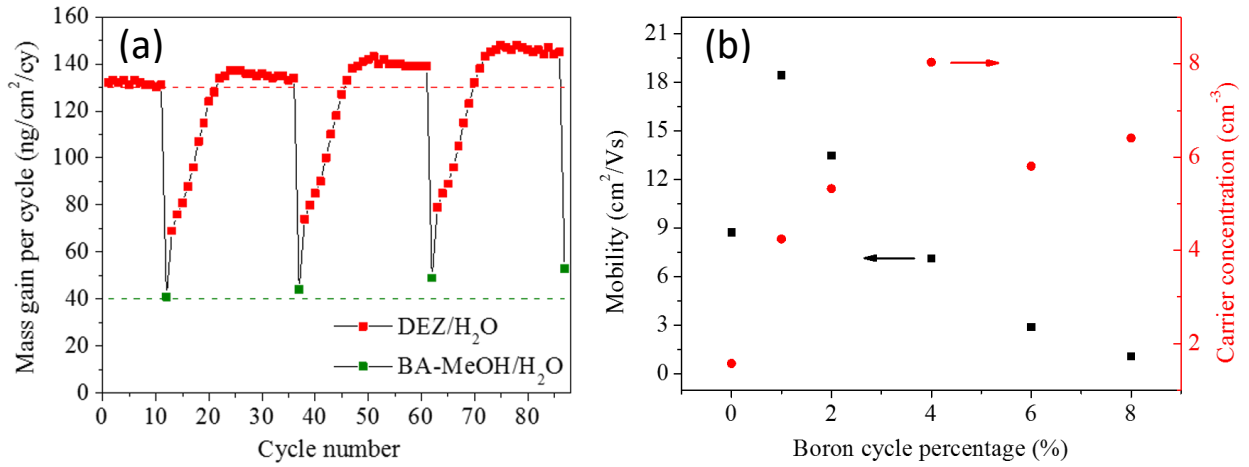
Figure 1: (a) QCM mass-uptake during ZnO:B ALD using 4% B-doping cycles, and (b) electrical transport properties for ZnO:B thin films versus B-doping cycle percentage.
