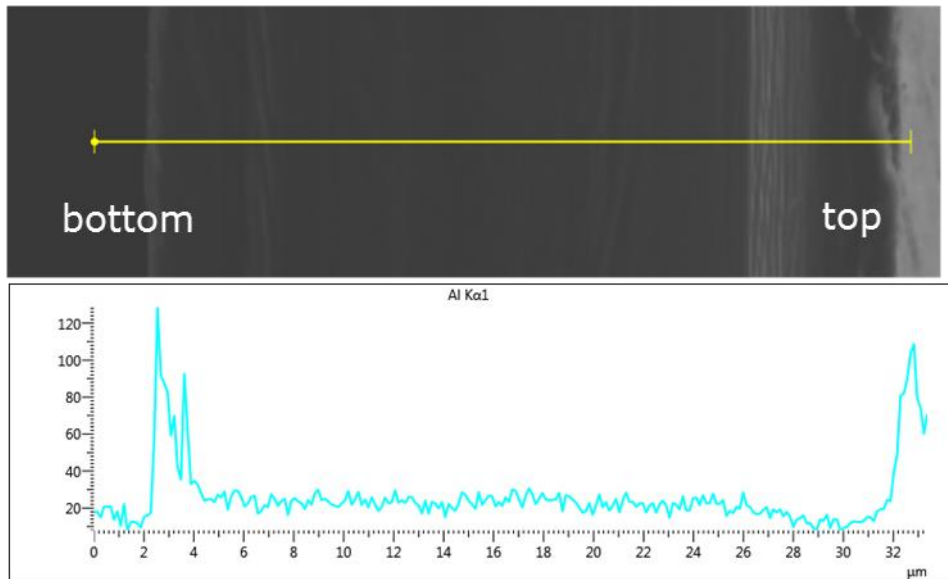
Figure 1. Cross-section SEM image of a Celgard® 2325 membrane coated with nominally 4 nm \text{Al}_2\text{O}_3 (40 cycles), with corresponding EDX line scan, showing a uniform coverage of aluminum across the porous structure.
