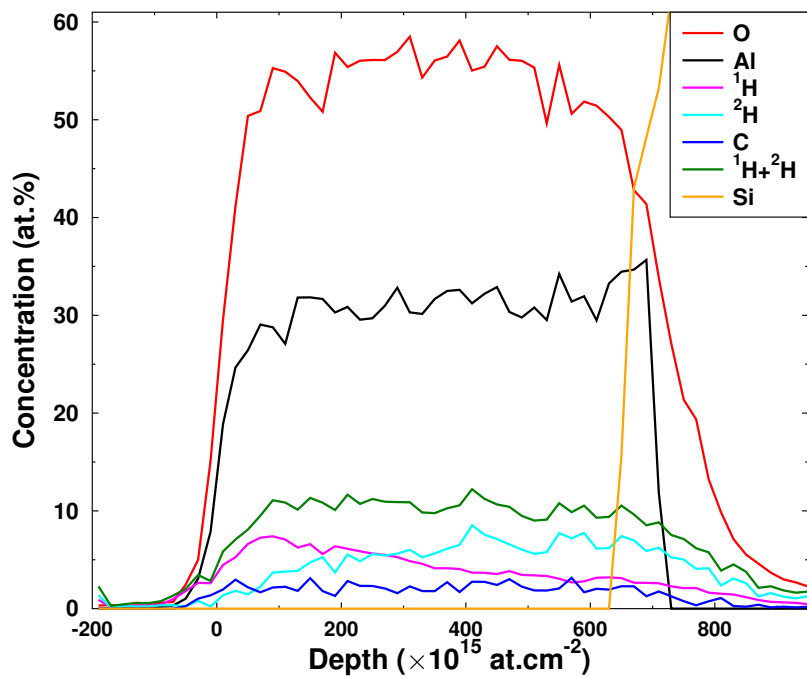
Figure 1. ToF-ERDA was used to measure elemental depth profile of aluminum oxide thin film deposited on silicon chip. Deposition temperature was 100 °C and TMA and D2O were used as precursors.
