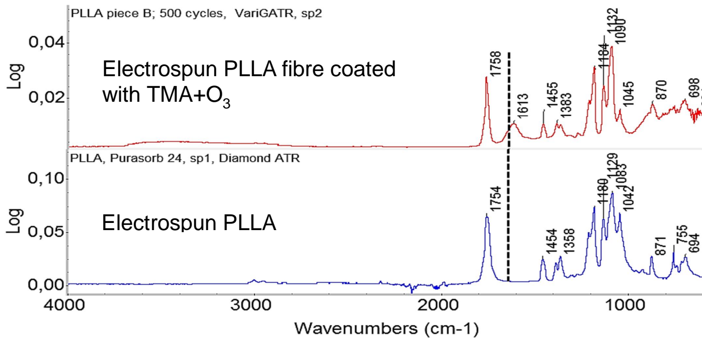
Figure 1. ATR-FTIR spectra of electrospun PLLA fibres and fibres coated with 500 cycles of Al 2 O 3 at 80°C.
