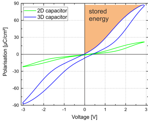
Fig 1: Polarisation-voltage hysteresis for 3D and 2D capacitors.
