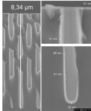
Fig 2: Step coverage of Si:HfO 2 applied for the formation of AFE capacitors.
