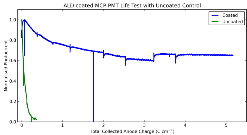
Figure 1. The difference between the lifetime and photocurrent generated for ALD coated and uncoated MCPs.
