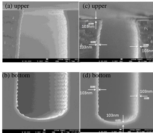
Fig. 2 (a), (b): Trench SEM images before deposition. (c), (d): Trench SEM images after AlO x deposition.
