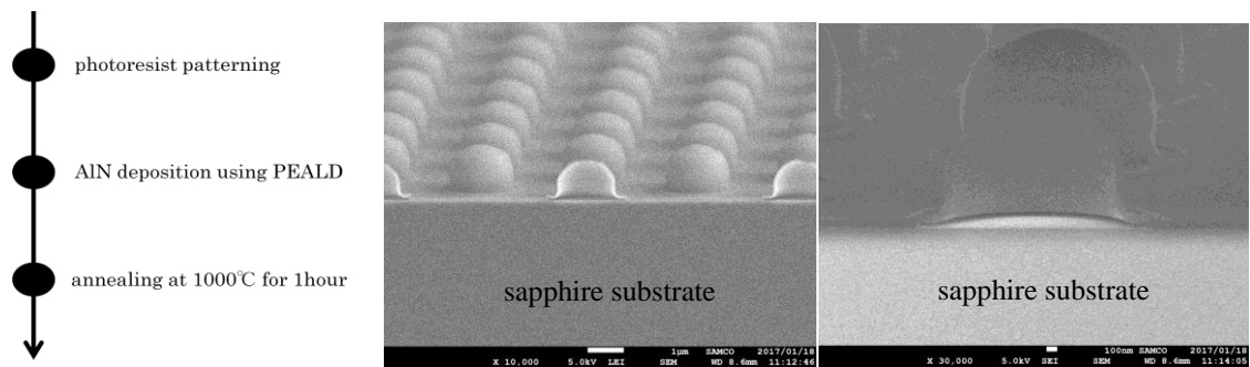
Fig.3 Process flow and SEM images of hollow structures.
