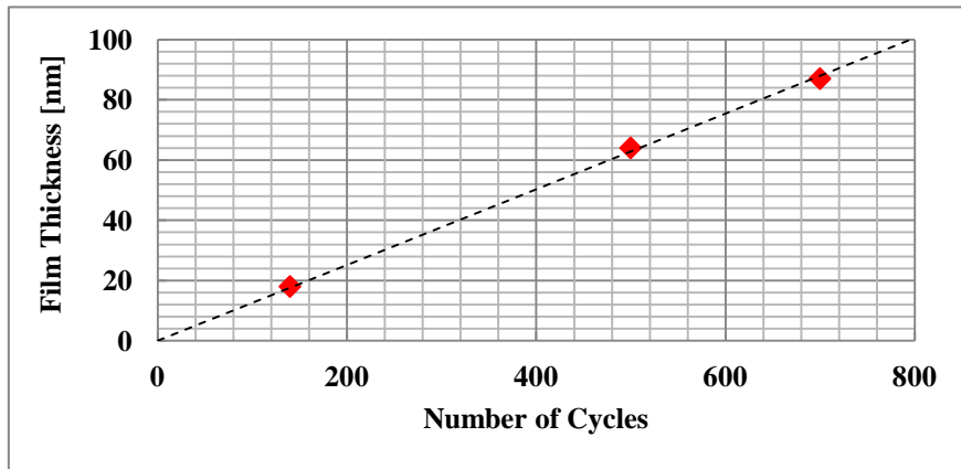
Fig.1 AlO x thickness versus number of process cycles.
