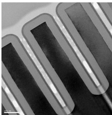
Fig.2. Step coverage of B-doped TiN
