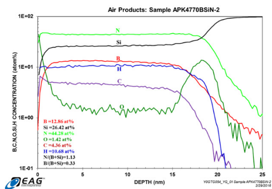
Fig.1 SIMS data of B-doped SiN
