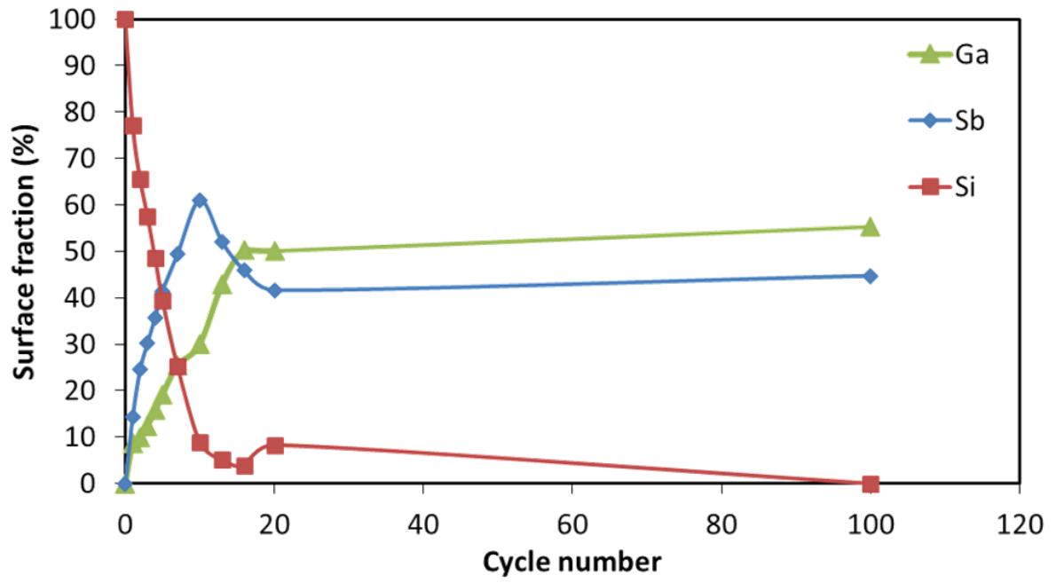
Fig. 1: Elemental surface fractions as a function of ALD cycle number.
