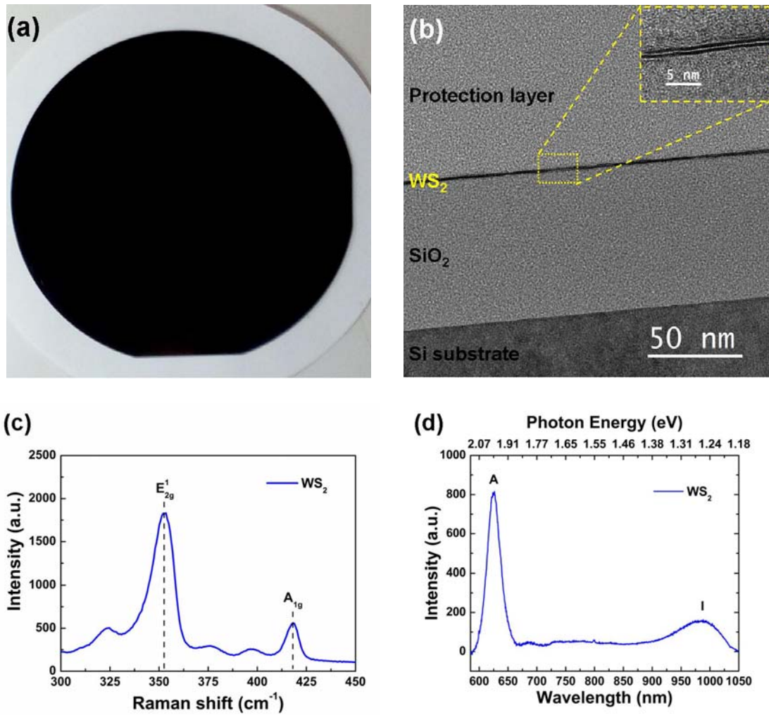
Figure 1. (a) A photograph of as-synthesized WS 2 film on 4-inch a Si/SiO 2 substrate. (b) Cross-sectional TEM image of high quality few-layer WS 2 on Si/SiO 2 substrate. (c) Raman spectrum of the wafer-scale WS 2 layers on Si/SiO 2 substrate. (d) PL spectrum of the wafer-scale WS 2 layers on Si/SiO 2 substrate.
