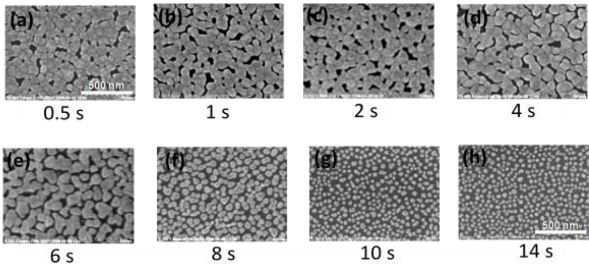
Nucleation as a function of purge pulse time, precursor pulse time = 2 s
