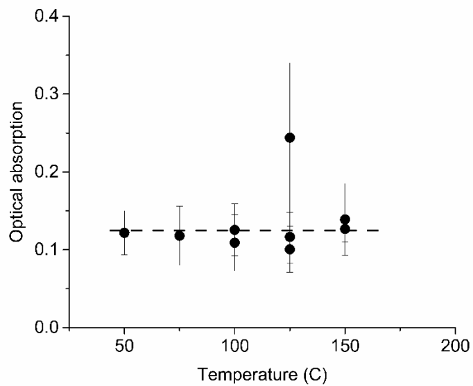
Film thickness (using exciton absorption as a proxy) as a function of deposition temperature showing the existence of an ALD window.
