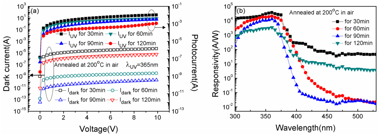
Fig.2 Dark- and photo-current characteristics (a) and spectral responsivity (b) of the ZnO MSM photodetectors annealed at 200°C in air for different time.
