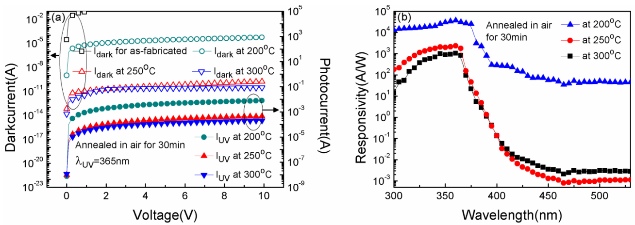
Fig.1 Dark- and photo-current characteristics (a) and spectral responsivity (b) of the ZnO MSM photodetectors annealed at different temperatures in air for 30min.
