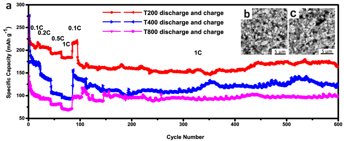
Figure 1. a) Rate and cycling performance of TiO 2 electrodes with different ALD cycles. SEM images of T200 electrode b) before and c) after all galvanostatic discharge/charge tests.
