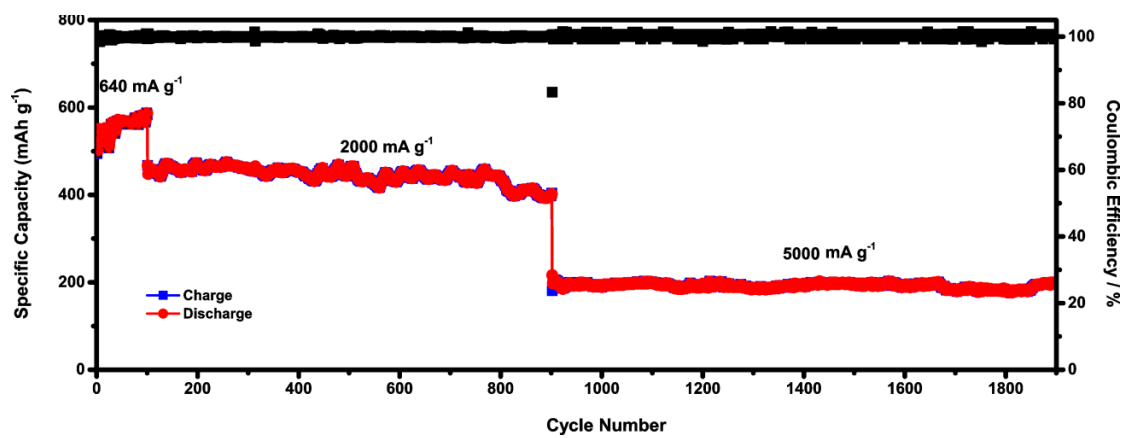
Figure 2. Rate and cycling performances of ZnO nanomembranes with 200 ALD cycles on carbon sponge.
