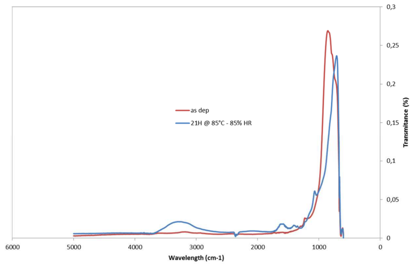
Figure 1. Evolution of IR spectra of alumina deposited at 80°C by exposition to humid atmosphere
