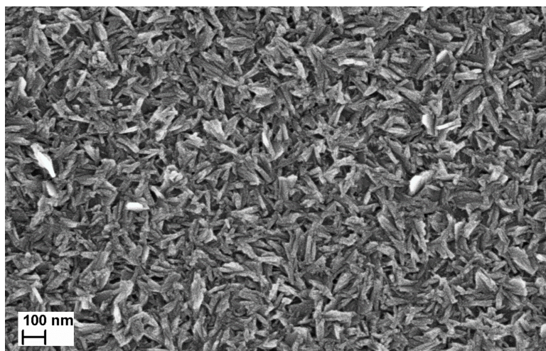
Figure 3. SEM image of alumina by exposition to humid atmosphere 24 hours at 85°C – 85% HR
