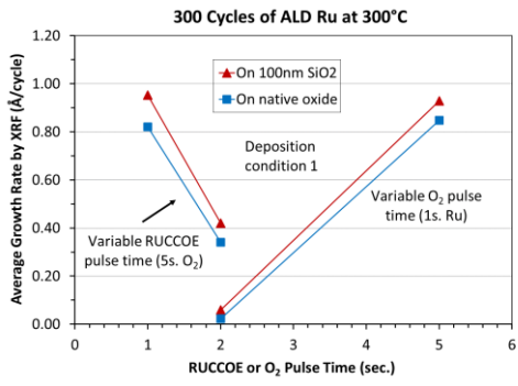
Figure 1. Average growth rate of Ru as measured by XRF as a function of the pulse time
