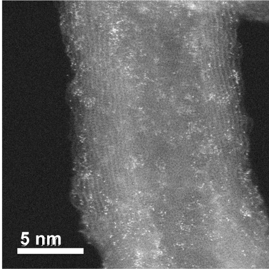
High resolution STEM image of single VO x sites on multi-walled carbon nanotubes.
